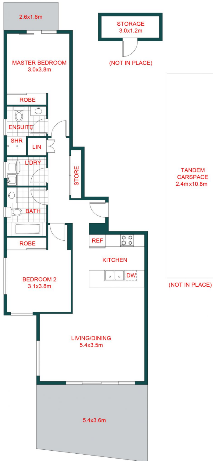
FLOOR PLAN
