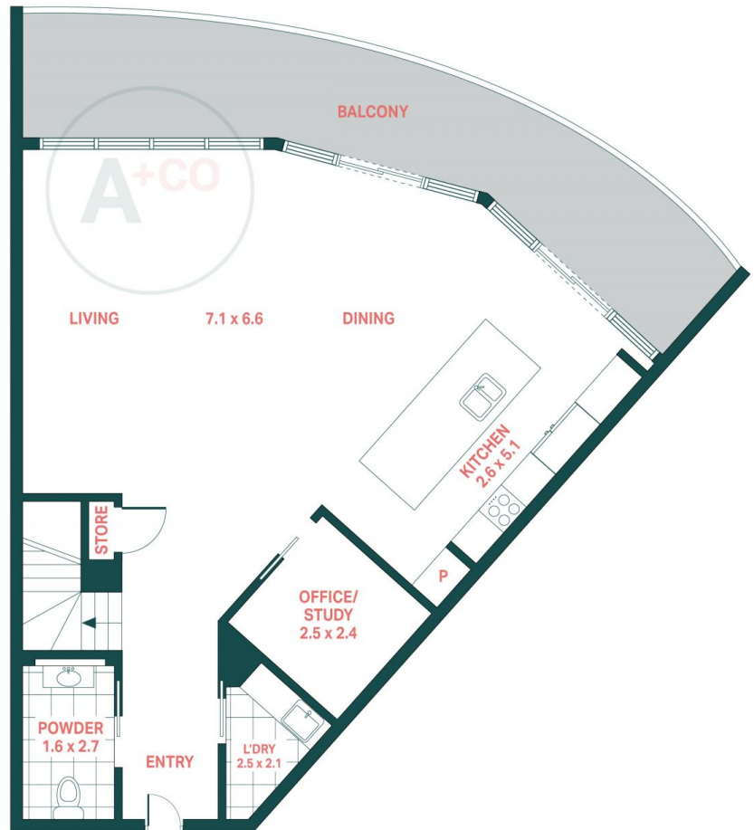
LOWER FLOOR
