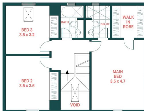
UPPER FLOOR
