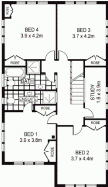
UPPER LEVEL
