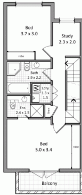
Level 1 floor plan
