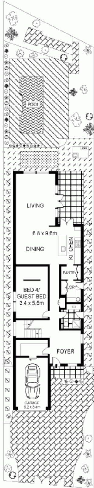
GROUND FLOOR
